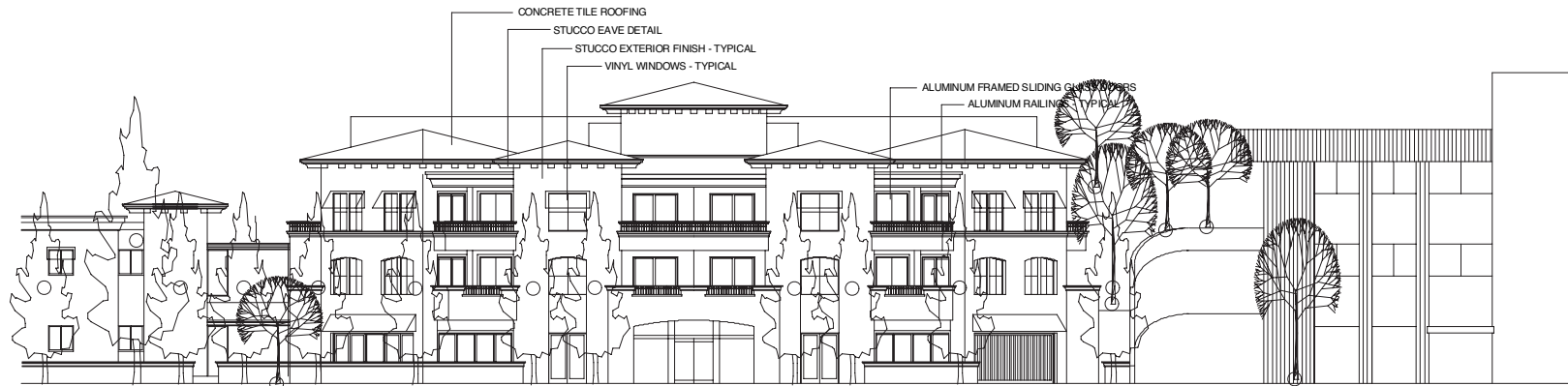
PENINSULA VILLAS NORTH ELEVATION
